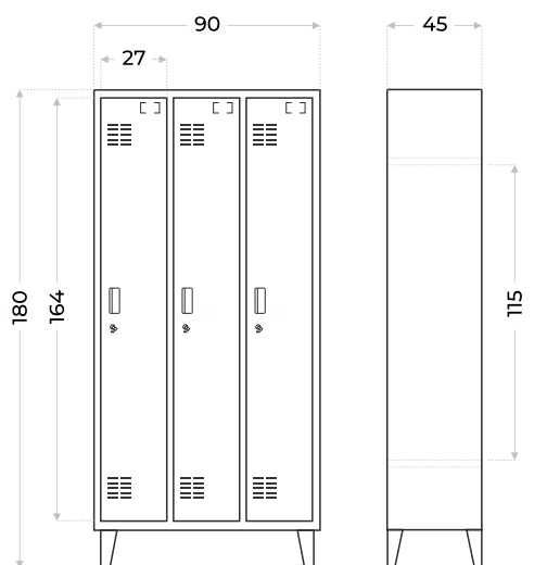
V. FRONTAL
