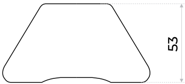
VISTA FRONTAL
